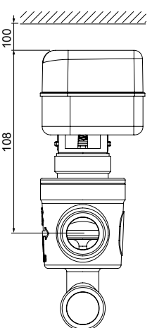
VTXT24P VTXT26P + MVT.03S
